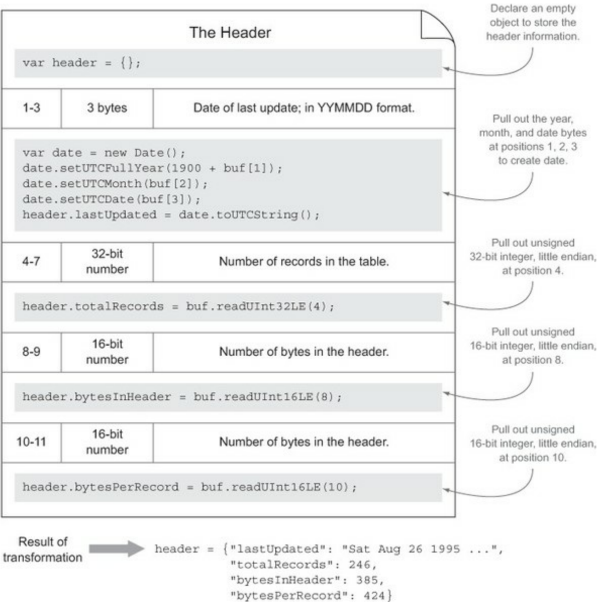
Figure 3.6. The header: transformation from the specification to code using the Node Buffer API
