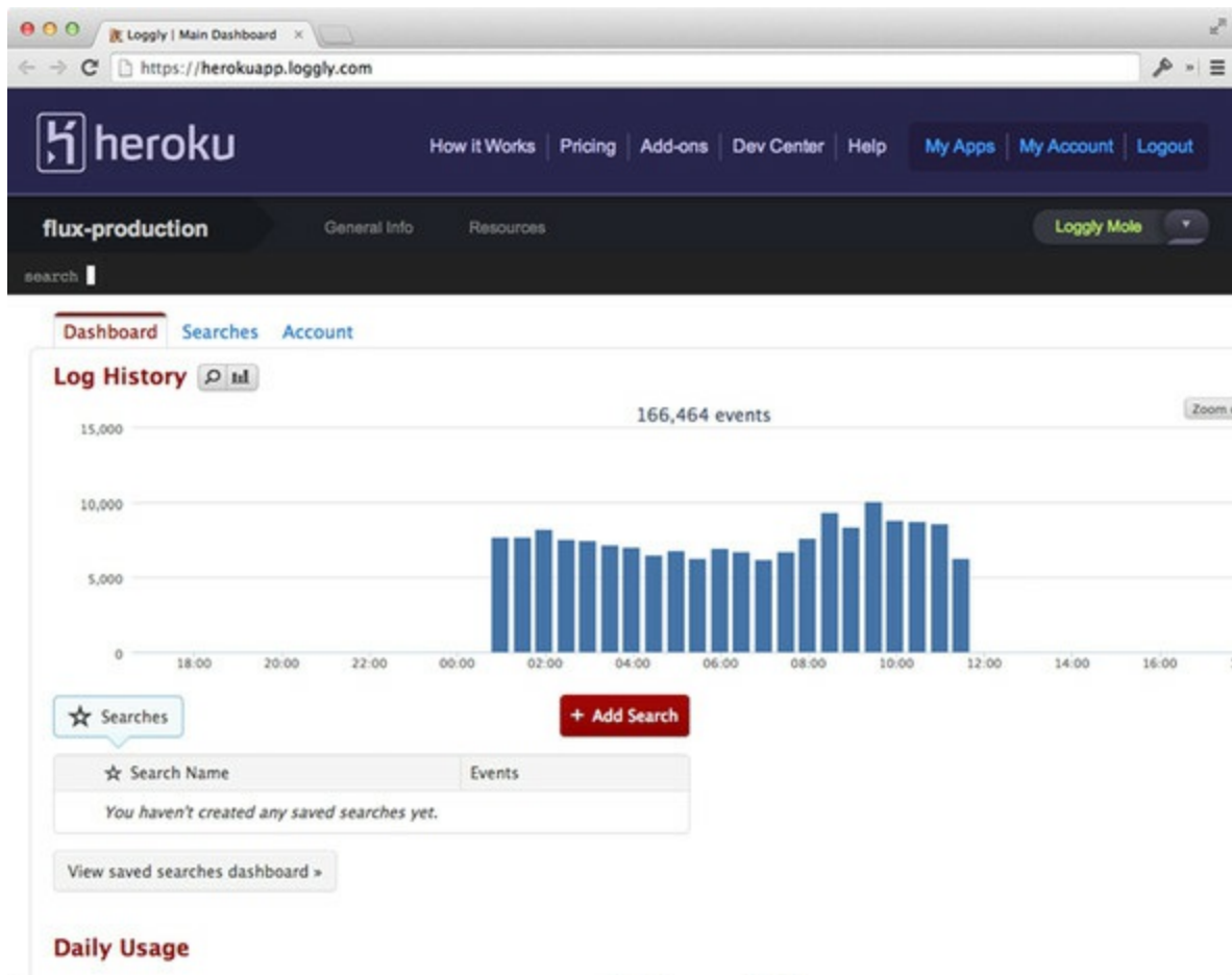
Figure 12.10. Loggly's dashboard
