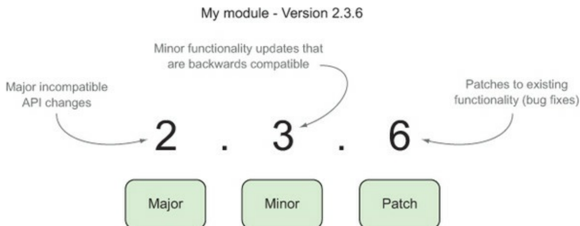
Figure 13.4. Semantic versioning
