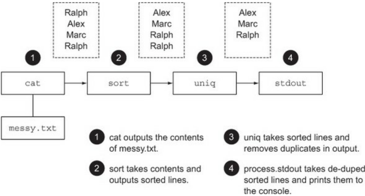
Figure 8.5. Stringing external applications together with spawn
