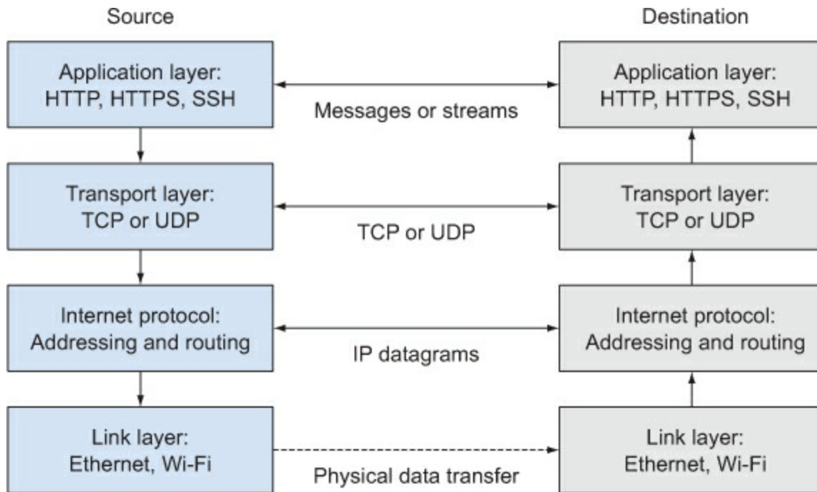
Figure 7.2. Network layer wrapping
