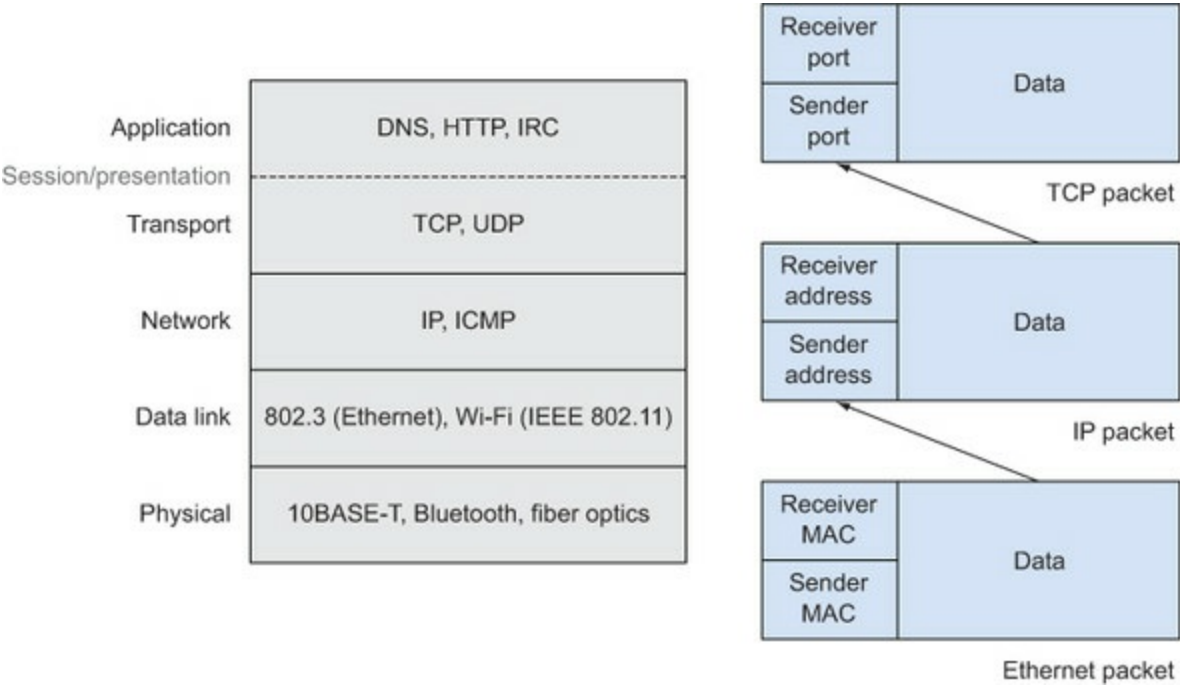
Figure 7.1. Protocols are grouped into seven logical layers. Packets are wrapped by protocols at consecutive layers.
